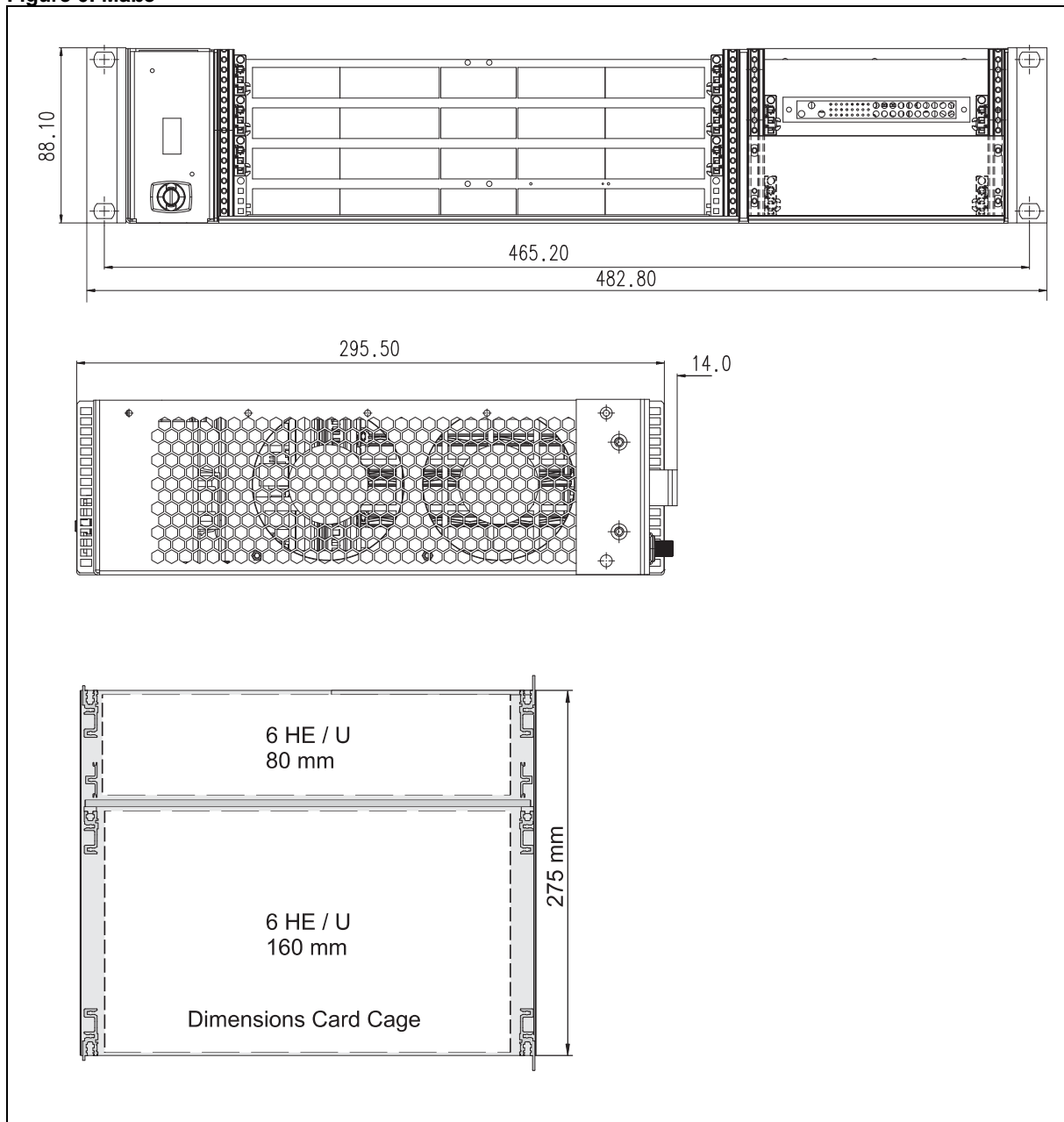
Figure 6: Maße
